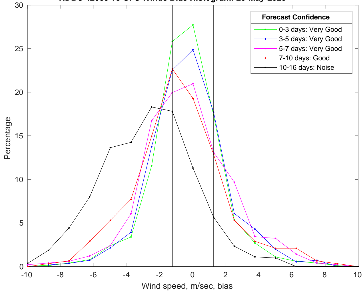
NDBC 42035 vs GFS Winds Bias Histogram: 20-May-2025
