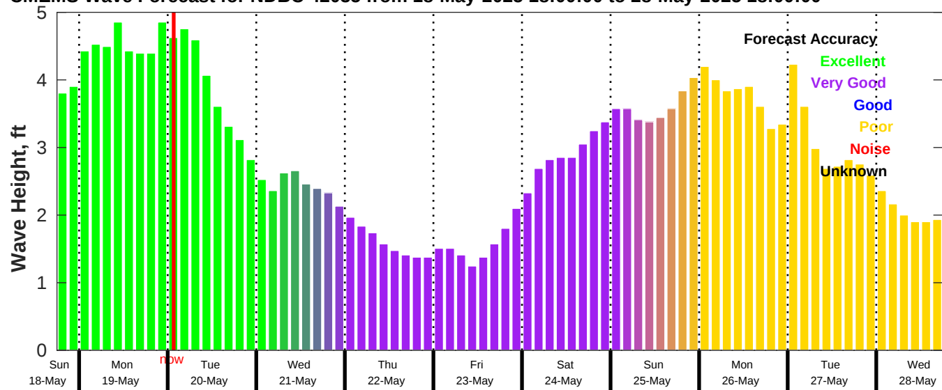
CMEMS Wave Forecast for NDBC 42035 from 18-May-2025 18:00:00 to 28-May-2025 18:00:00
