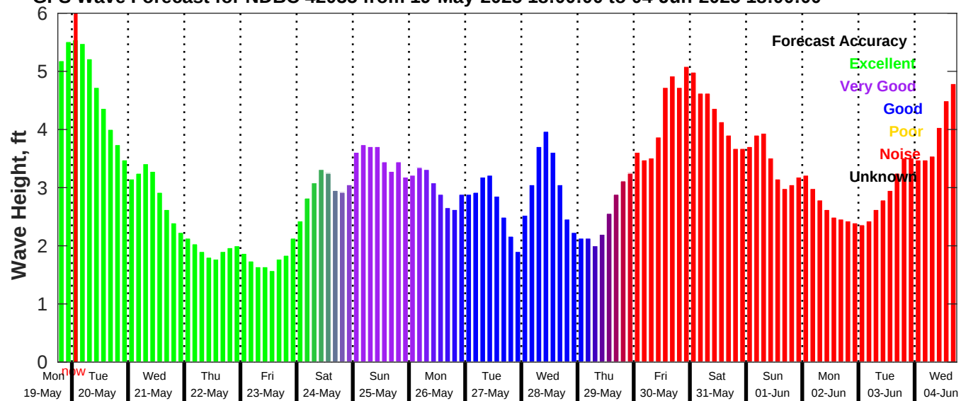
GFS Wave Forecast for NDBC 42035 from 19-May-2025 18:00:00 to 04-Jun-2025 18:00:00
