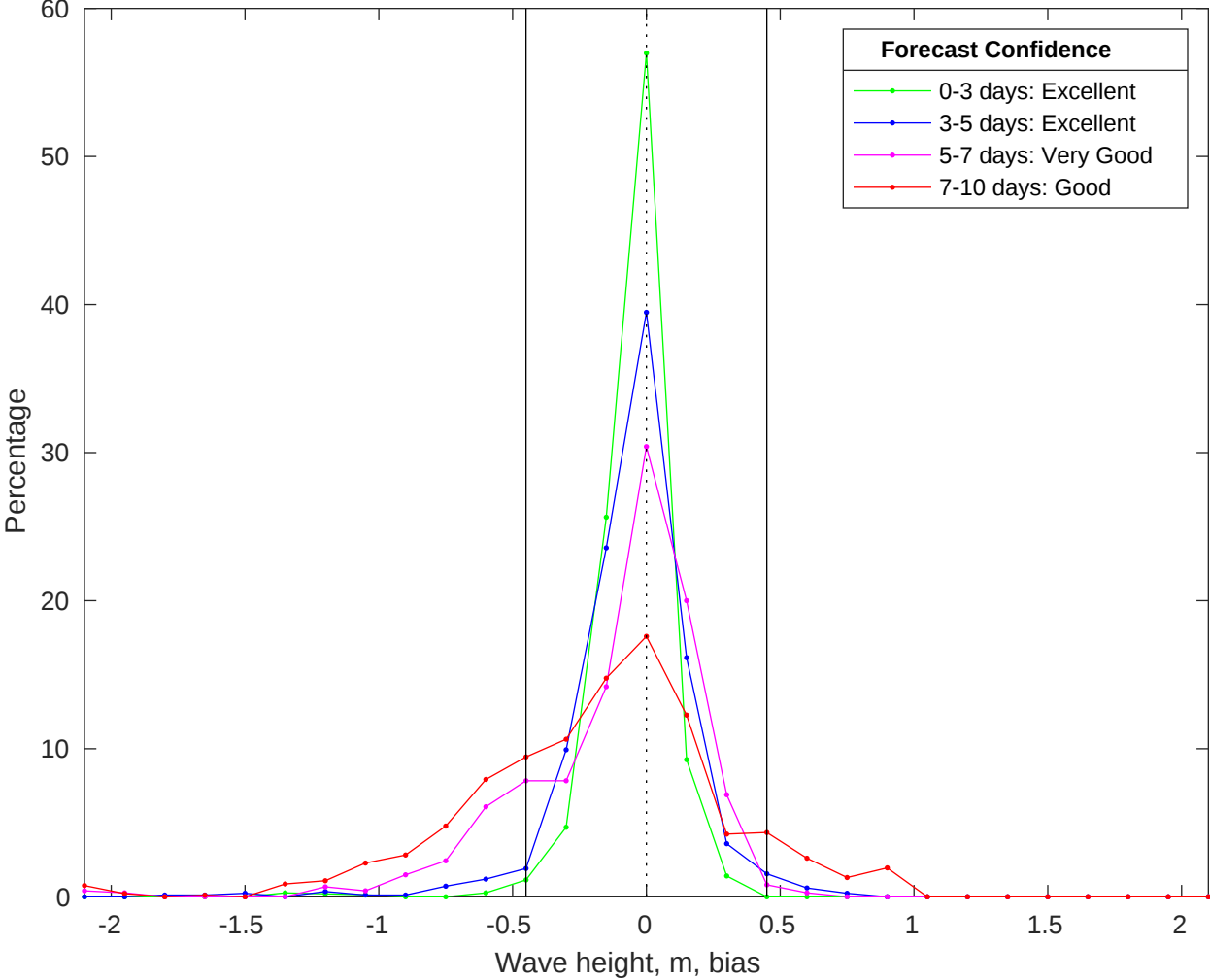
NDBC 42036 vs CMEMS Waves Bias Histogram: 20-May-2025
