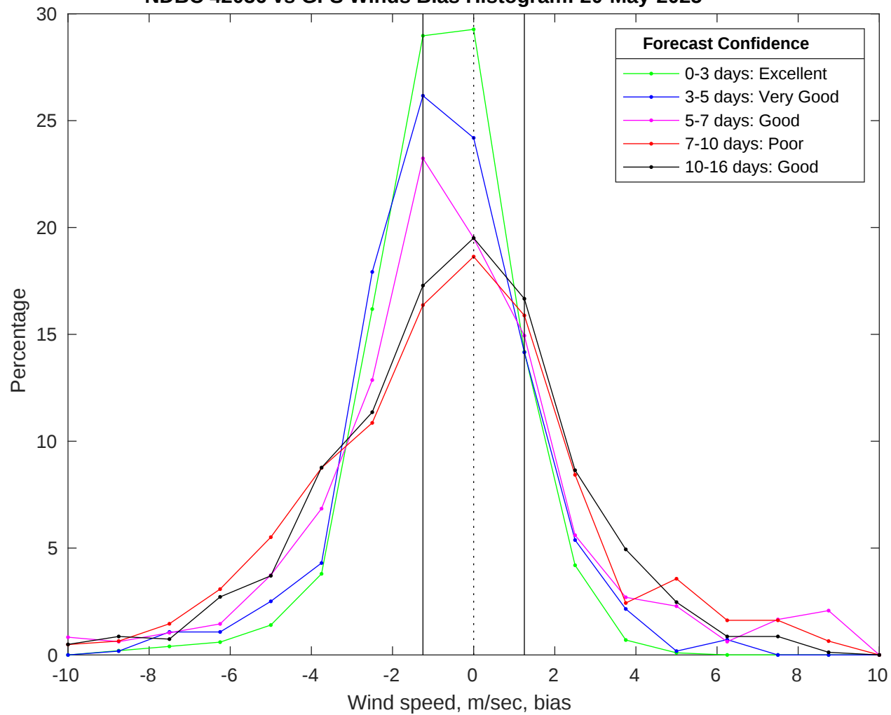
NDBC 42036 vs GFS Winds Bias Histogram: 20-May-2025
