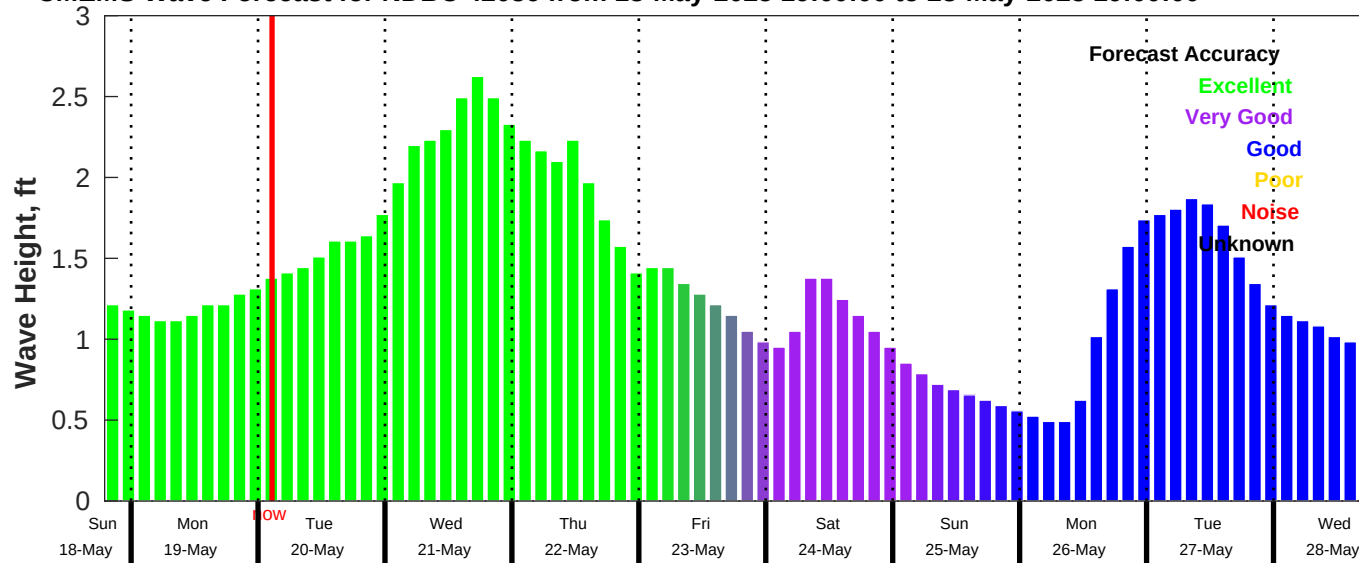
CMEMS Wave Forecast for NDBC 42036 from 18-May-2025 19:00:00 to 28-May-2025 19:00:00
