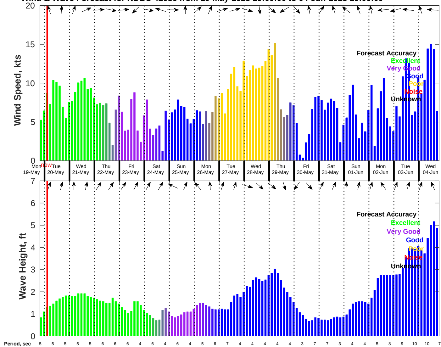
Wind & Wave Forecast for NDBC 42036 from 19-May-2025 19:00:00 to 04-Jun-2025 19:00:00
