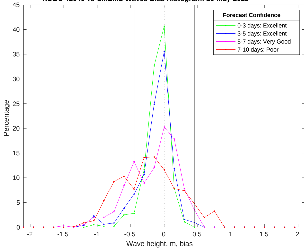
NDBC 42040 vs CMEMS Waves Bias Histogram: 20-May-2025
