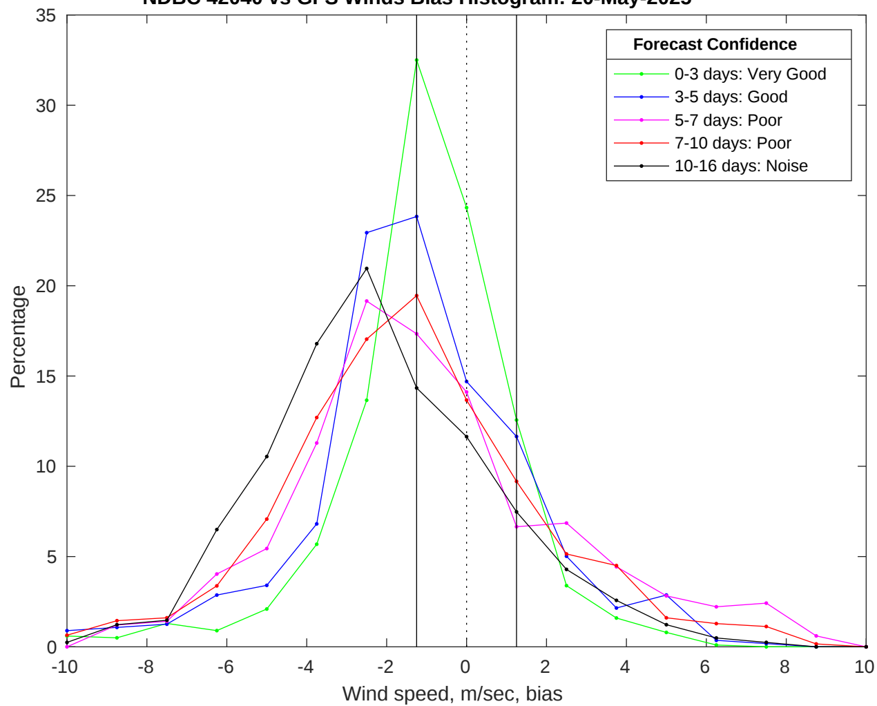
NDBC 42040 vs GFS Winds Bias Histogram: 20-May-2025
