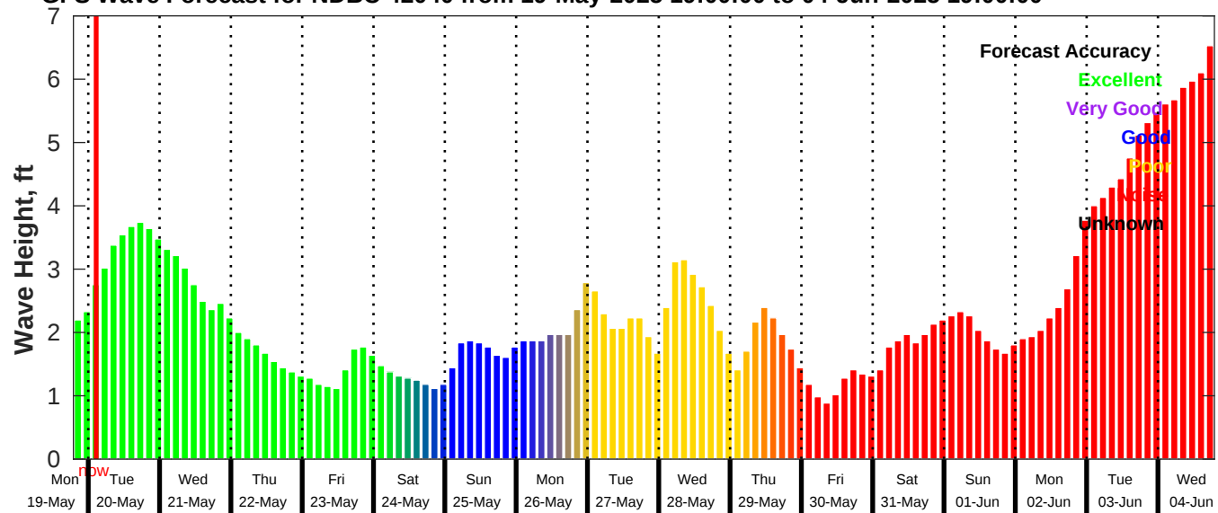
GFS Wave Forecast for NDBC 42040 from 19-May-2025 19:00:00 to 04-Jun-2025 19:00:00
