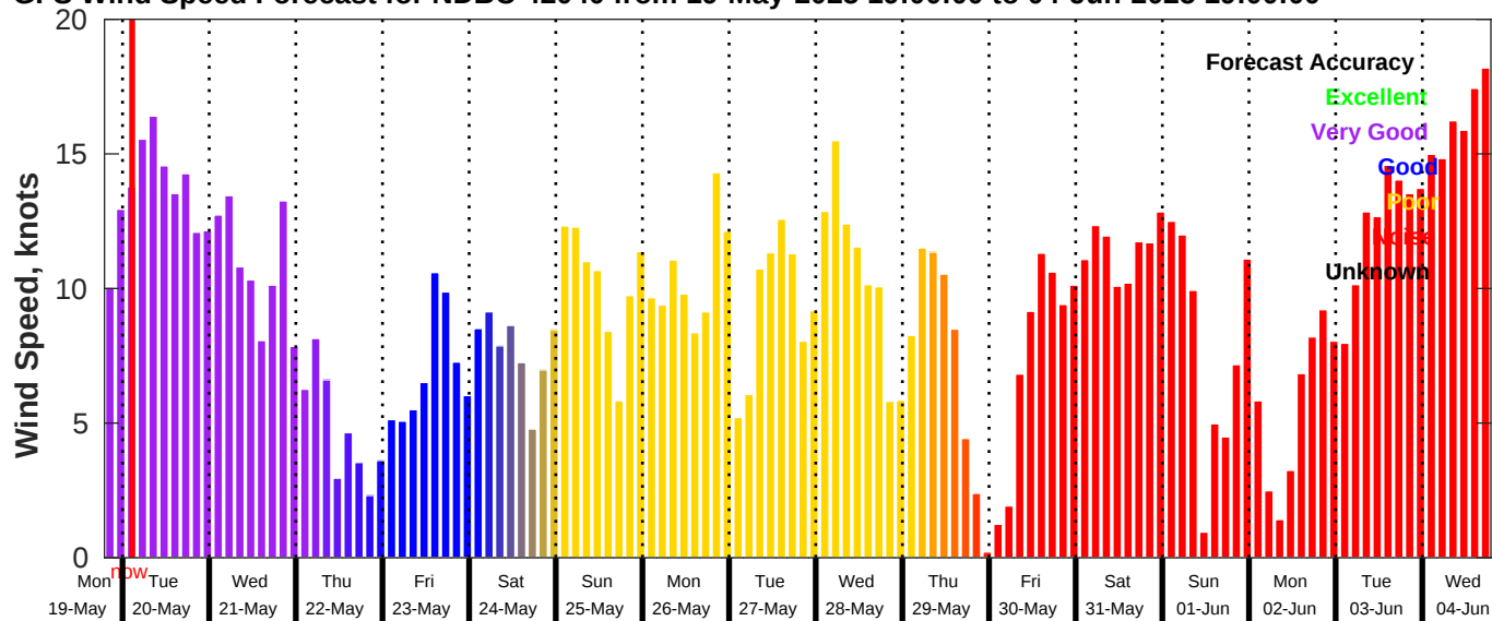
GFS Wind Speed Forecast for NDBC 42040 from 19-May-2025 19:00:00 to 04-Jun-2025 19:00:00
