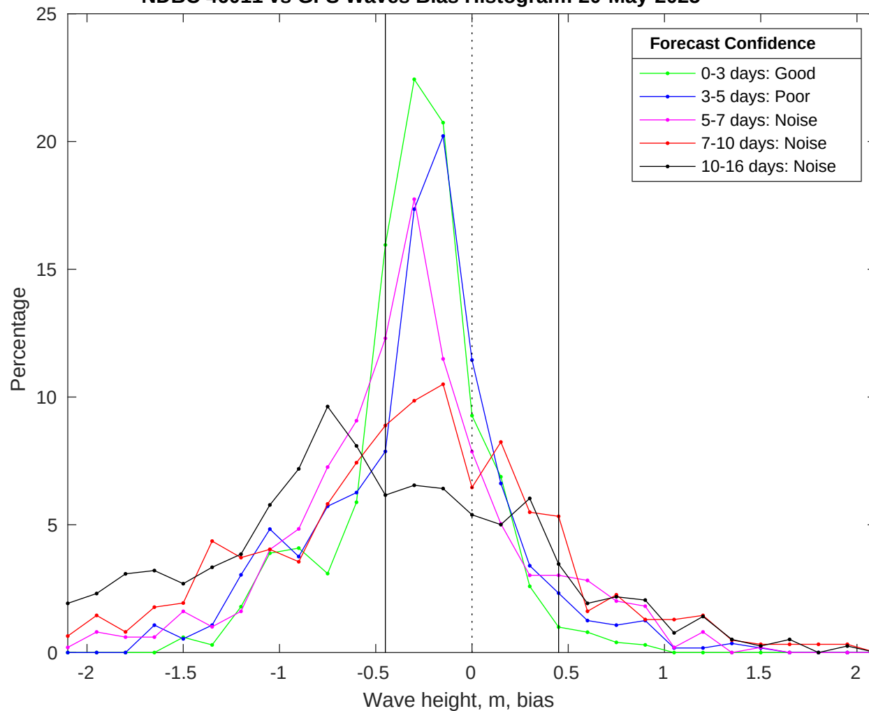
NDBC 46011 vs GFS Waves Bias Histogram: 20-May-2025
