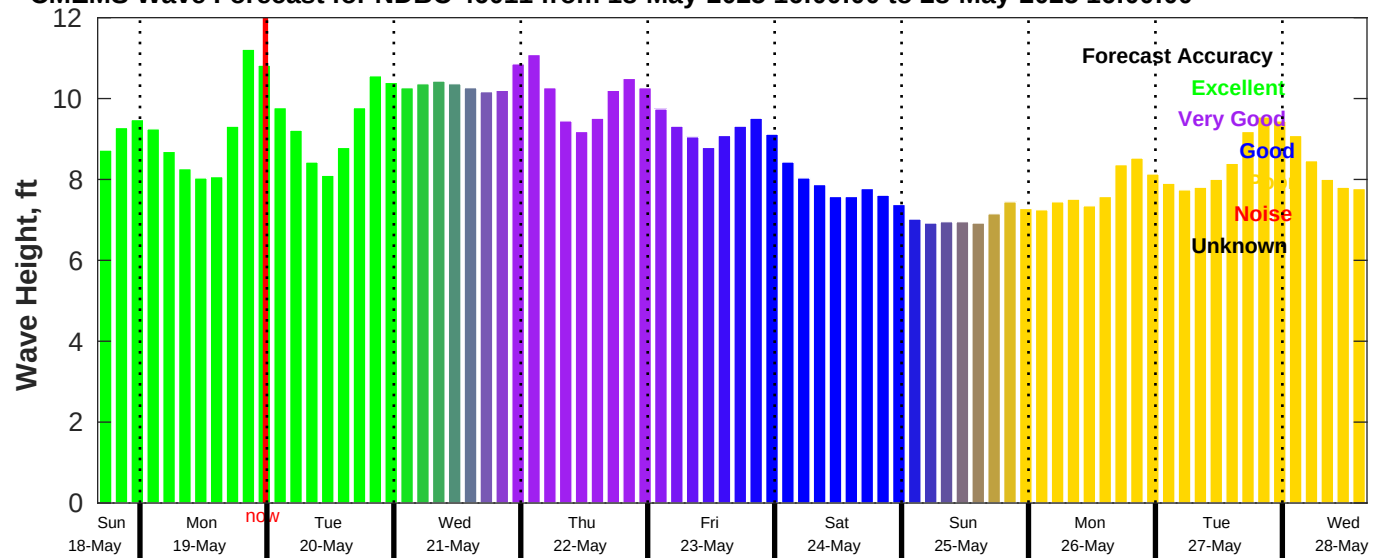
CMEMS Wave Forecast for NDBC 46011 from 18-May-2025 16:00:00 to 28-May-2025 16:00:00
