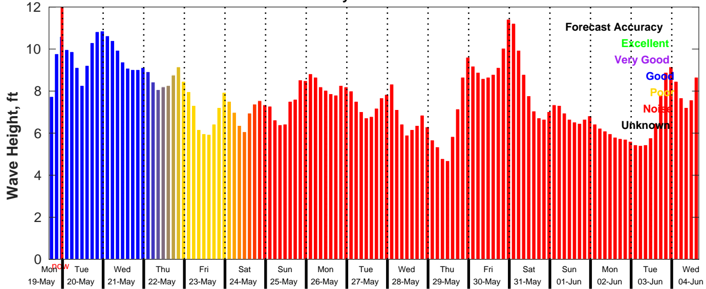
GFS Wave Forecast for NDBC 46011 from 19-May-2025 16:00:00 to 04-Jun-2025 16:00:00
