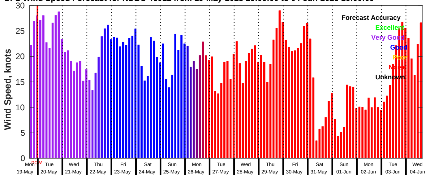
GFS Wind Speed Forecast for NDBC 46011 from 19-May-2025 16:00:00 to 04-Jun-2025 16:00:00
