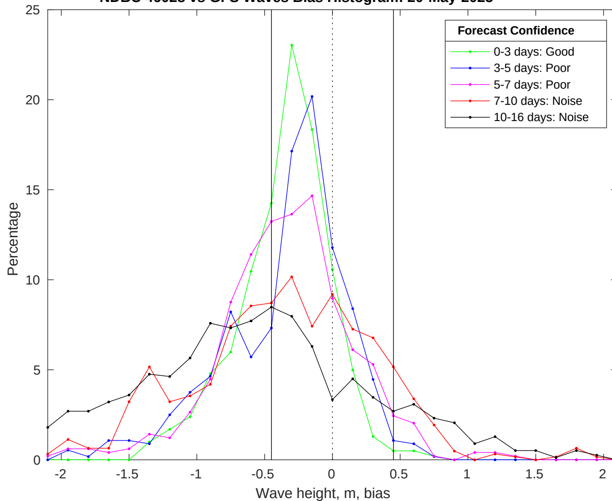
NDBC 46028 vs GFS Waves Bias Histogram: 20-May-2025
