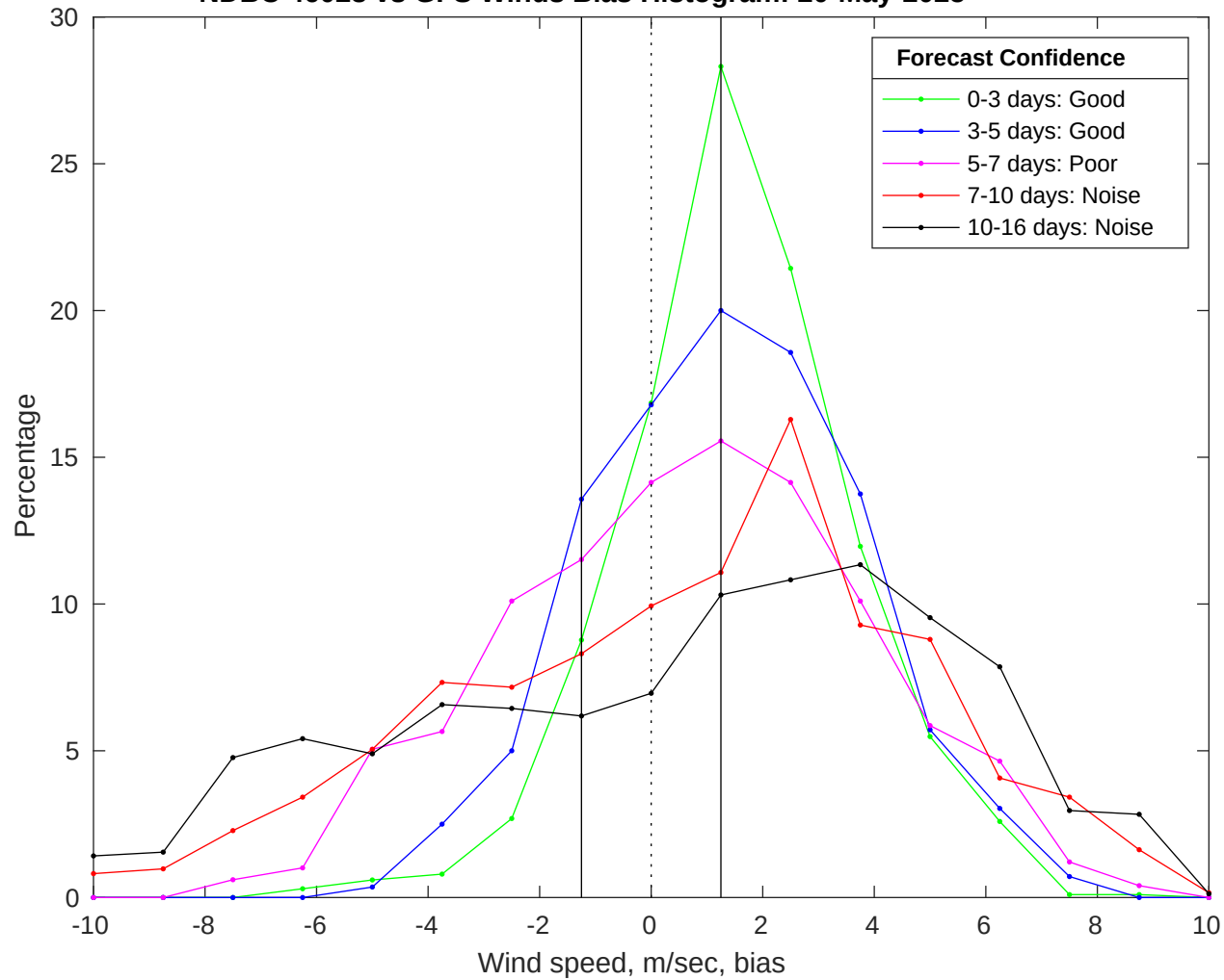
NDBC 46028 vs GFS Winds Bias Histogram: 20-May-2025
