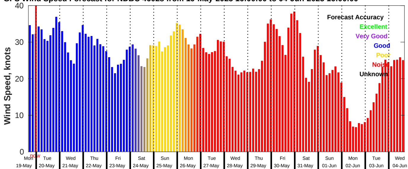
GFS Wind Speed Forecast for NDBC 46028 from 19-May-2025 16:00:00 to 04-Jun-2025 16:00:00
