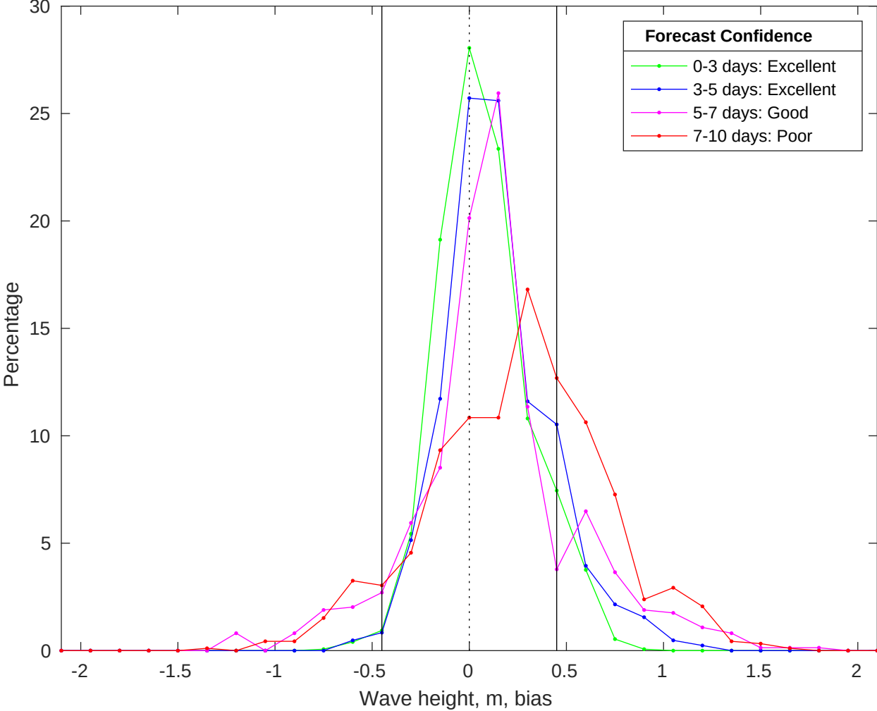
NDBC 46054 vs CMEMS Waves Bias Histogram: 20-May-2025
