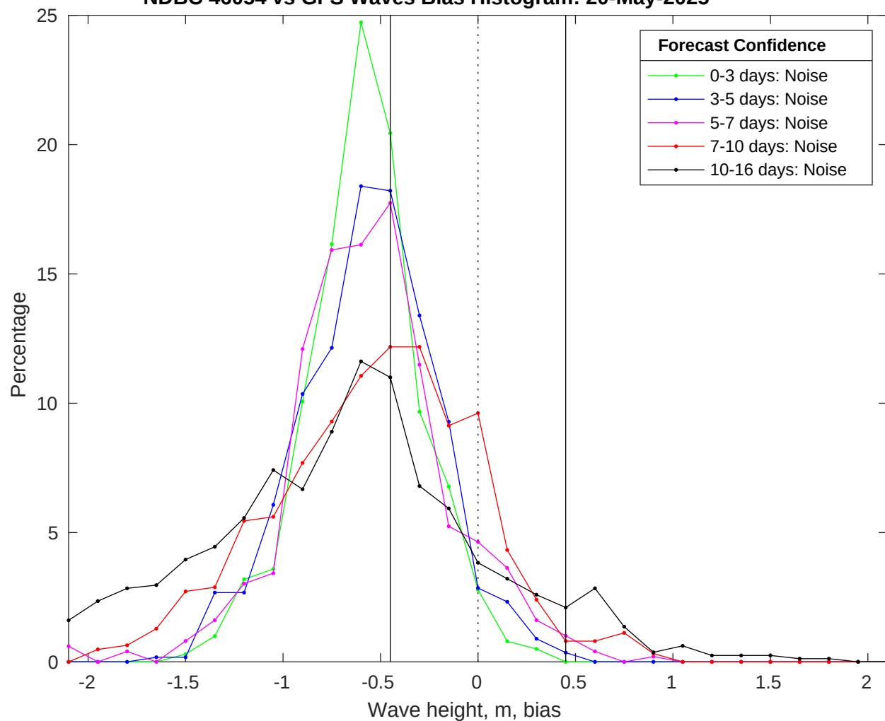
NDBC 46054 vs GFS Waves Bias Histogram: 20-May-2025
