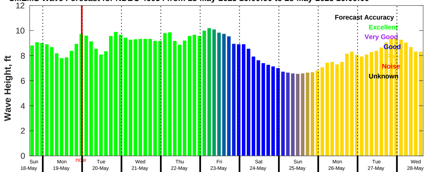
CMEMS Wave Forecast for NDBC 46054 from 18-May-2025 16:00:00 to 28-May-2025 16:00:00
