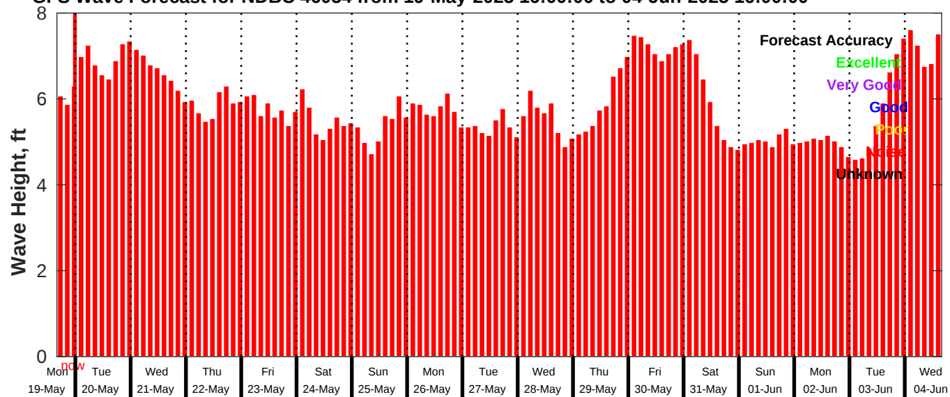
GFS Wave Forecast for NDBC 46054 from 19-May-2025 16:00:00 to 04-Jun-2025 16:00:00
