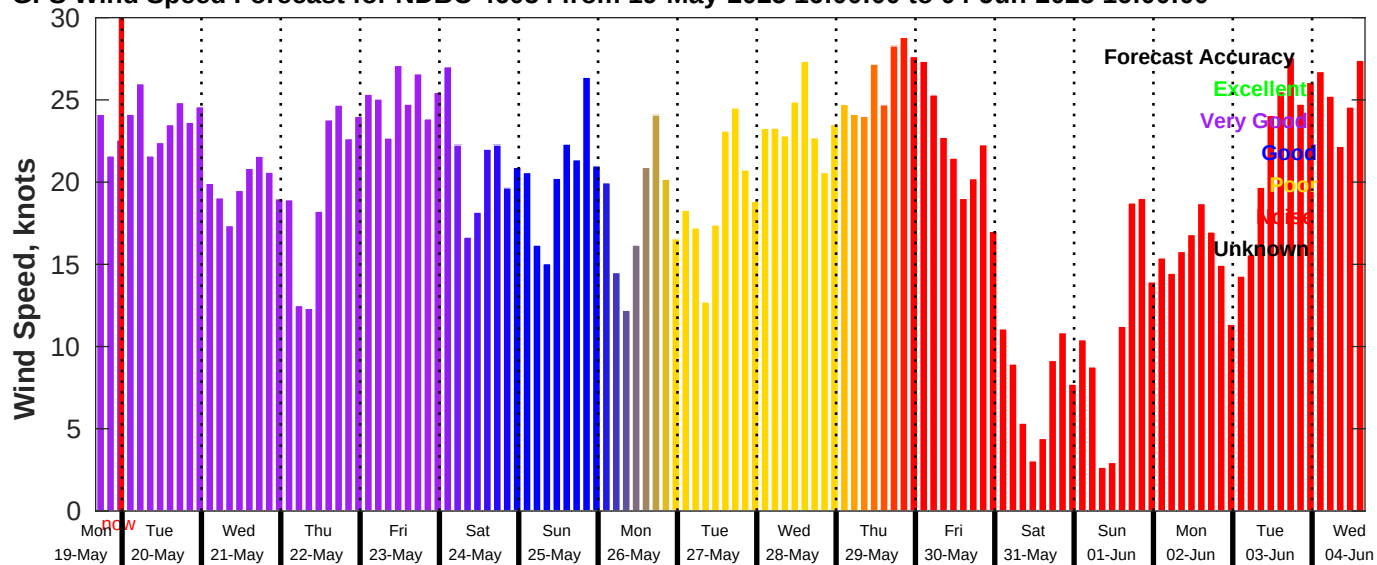
GFS Wind Speed Forecast for NDBC 46054 from 19-May-2025 16:00:00 to 04-Jun-2025 16:00:00
