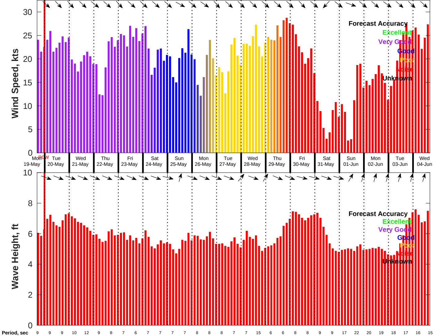
Wind & Wave Forecast for NDBC 46054 from 19-May-2025 16:00:00 to 04-Jun-2025 16:00:00
