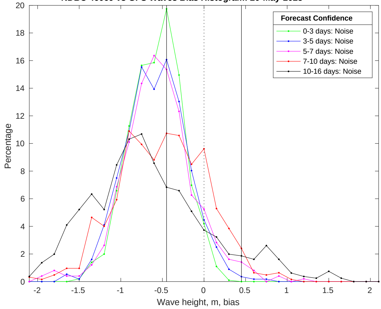
NDBC 46069 vs GFS Waves Bias Histogram: 20-May-2025
