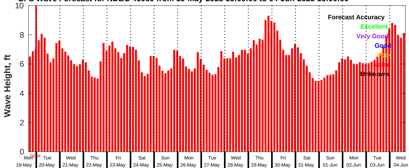
GFS Wave Forecast for NDBC 46069 from 19-May-2025 16:00:00 to 04-Jun-2025 16:00:00
