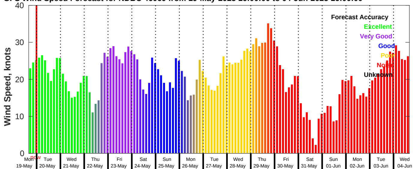
GFS Wind Speed Forecast for NDBC 46069 from 19-May-2025 16:00:00 to 04-Jun-2025 16:00:00
