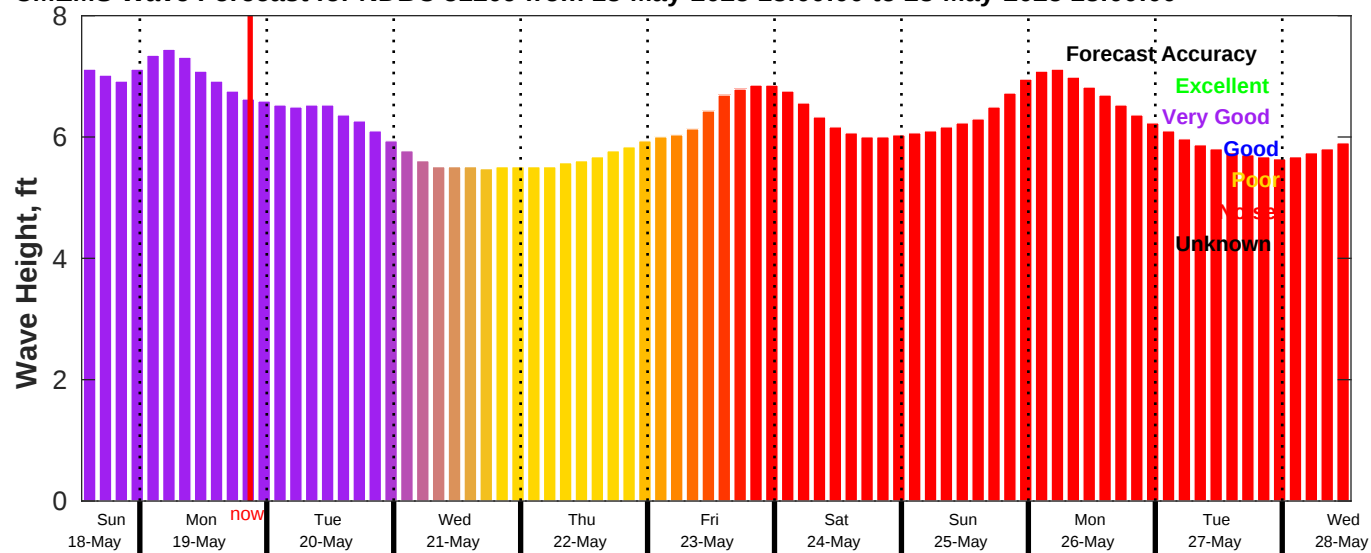
CMEMS Wave Forecast for NDBC 51209 from 18-May-2025 13:00:00 to 28-May-2025 13:00:00
