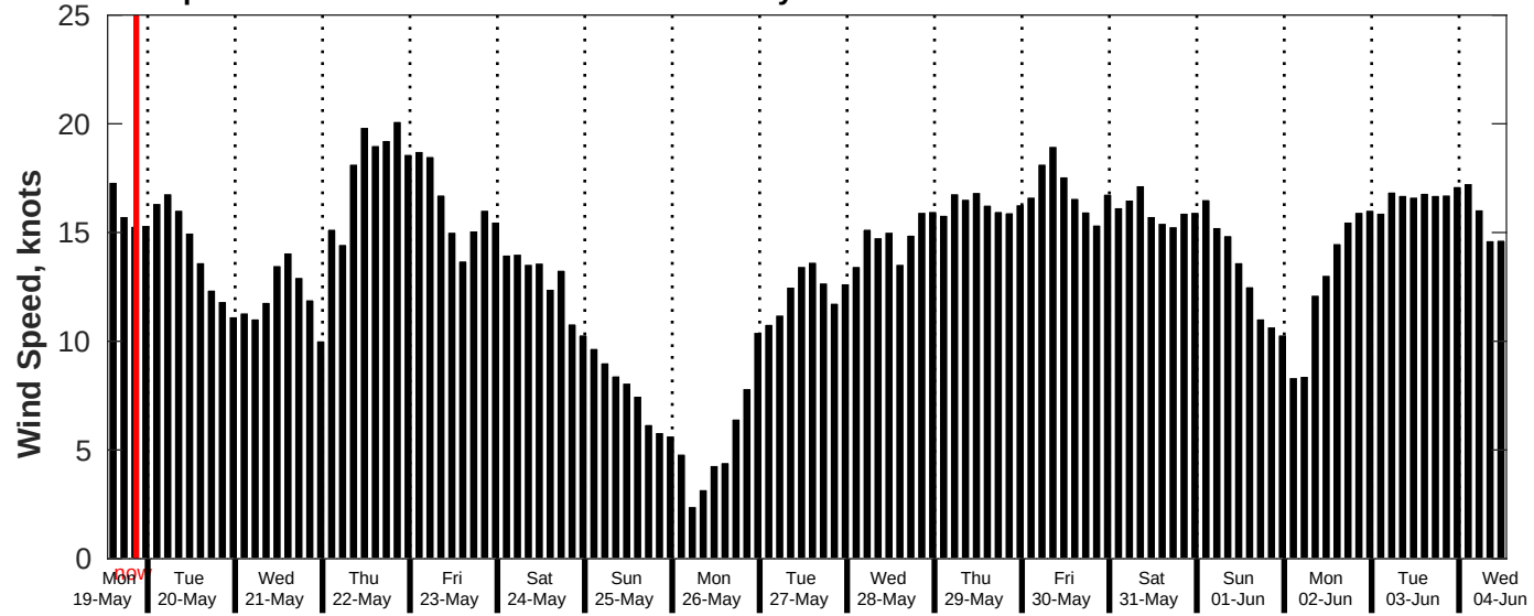
GFS Wind Speed Forecast for NDBC 51209 from 19-May-2025 13:00:00 to 04-Jun-2025 13:00:00
