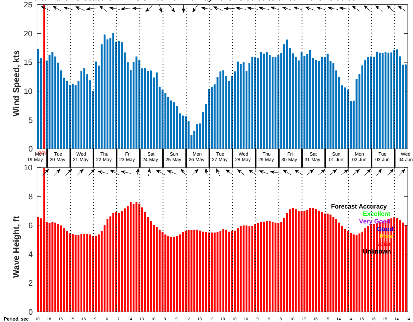
Wind & Wave Forecast for NDBC 51209 from 19-May-2025 13:00:00 to 04-Jun-2025 13:00:00
