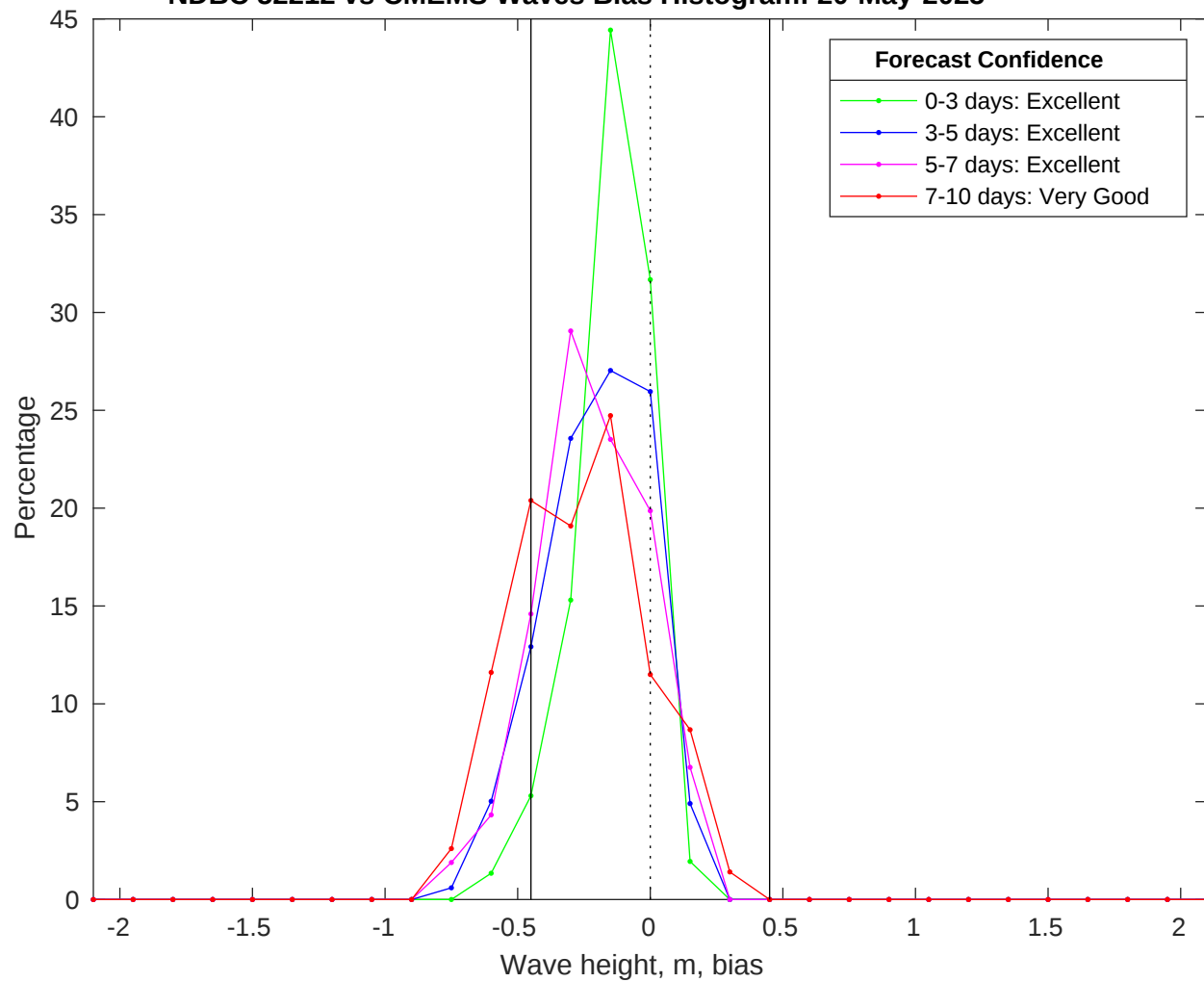
NDBC 52212 vs CMEMS Waves Bias Histogram: 20-May-2025
