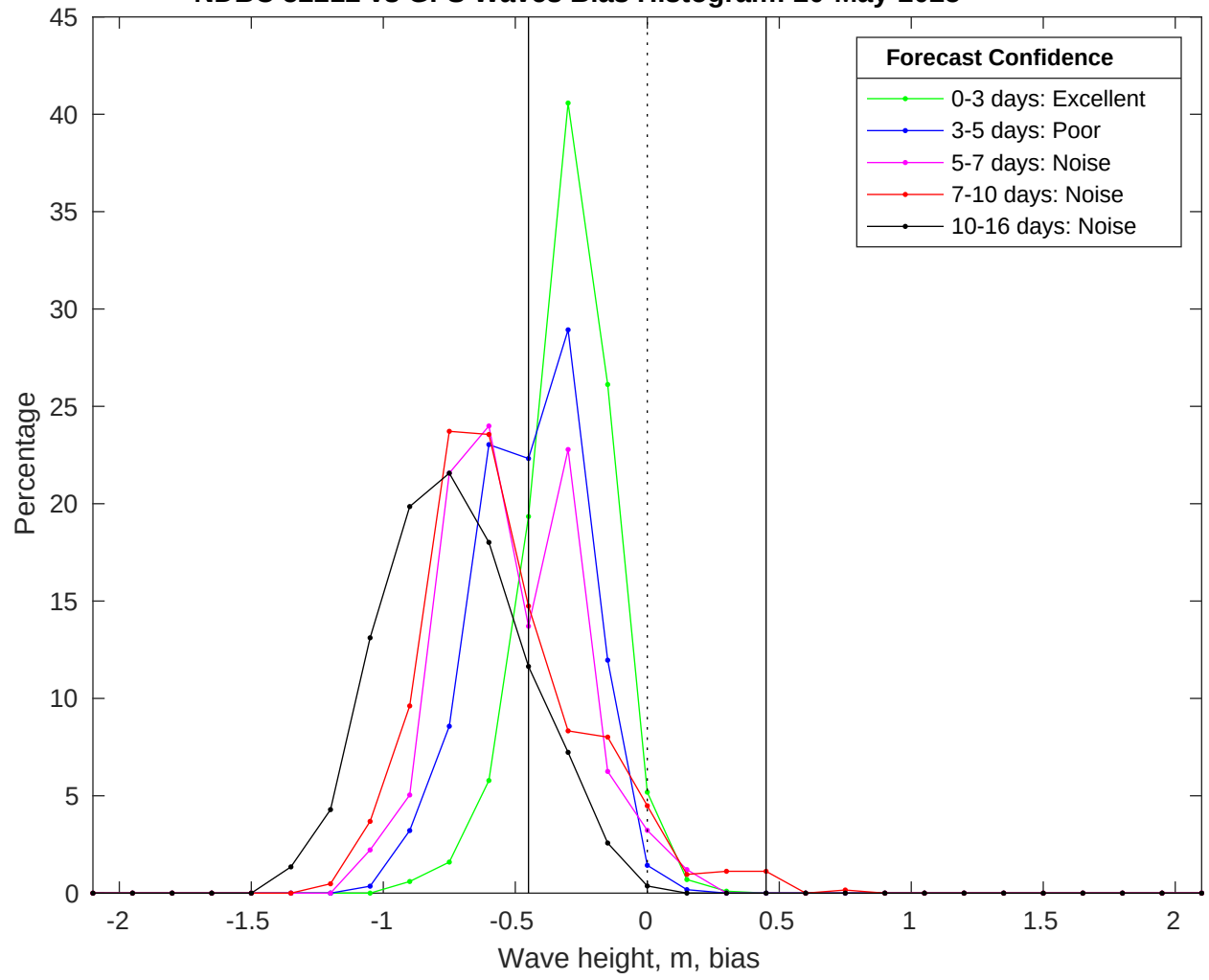
NDBC 52212 vs GFS Waves Bias Histogram: 20-May-2025
