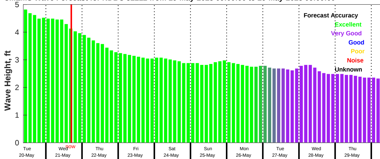
CMEMS Wave Forecast for NDBC 52212 from 19-May-2025 09:00:00 to 29-May-2025 09:00:00
