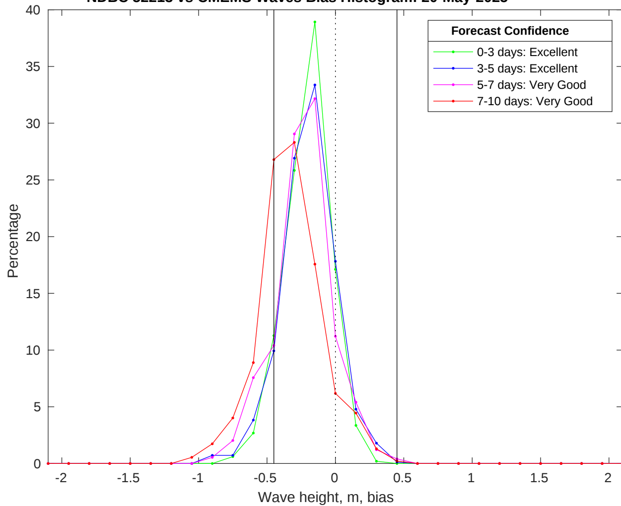
NDBC 52213 vs CMEMS Waves Bias Histogram: 20-May-2025
