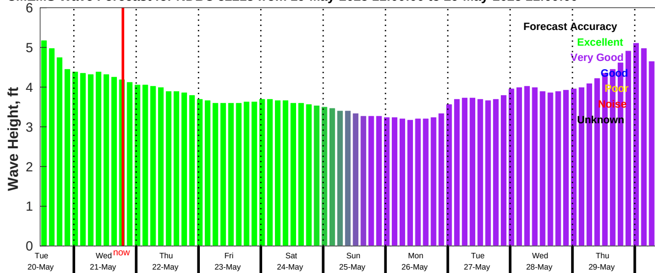
CMEMS Wave Forecast for NDBC 52213 from 19-May-2025 11:00:00 to 29-May-2025 11:00:00
