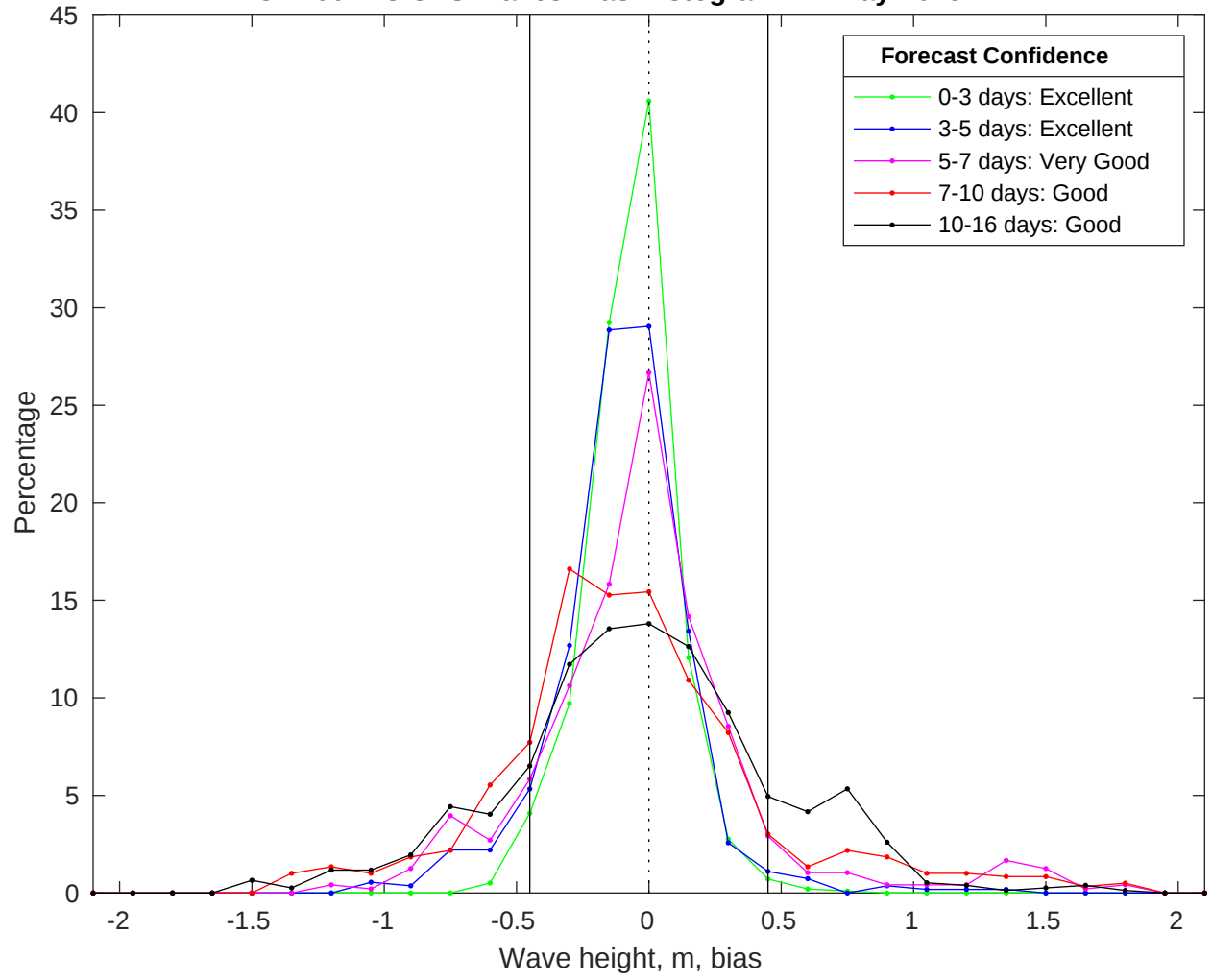
NDBC 41004 vs GFS Waves Bias Histogram: 21-May-2025
