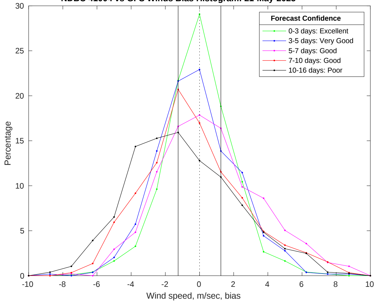
NDBC 41004 vs GFS Winds Bias Histogram: 21-May-2025
