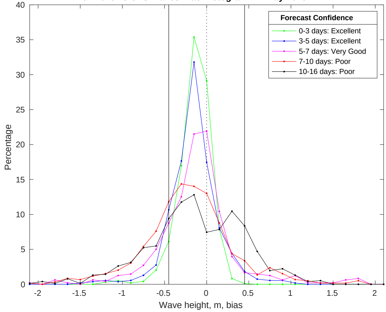
NDBC 41013 vs GFS Waves Bias Histogram: 21-May-2025
