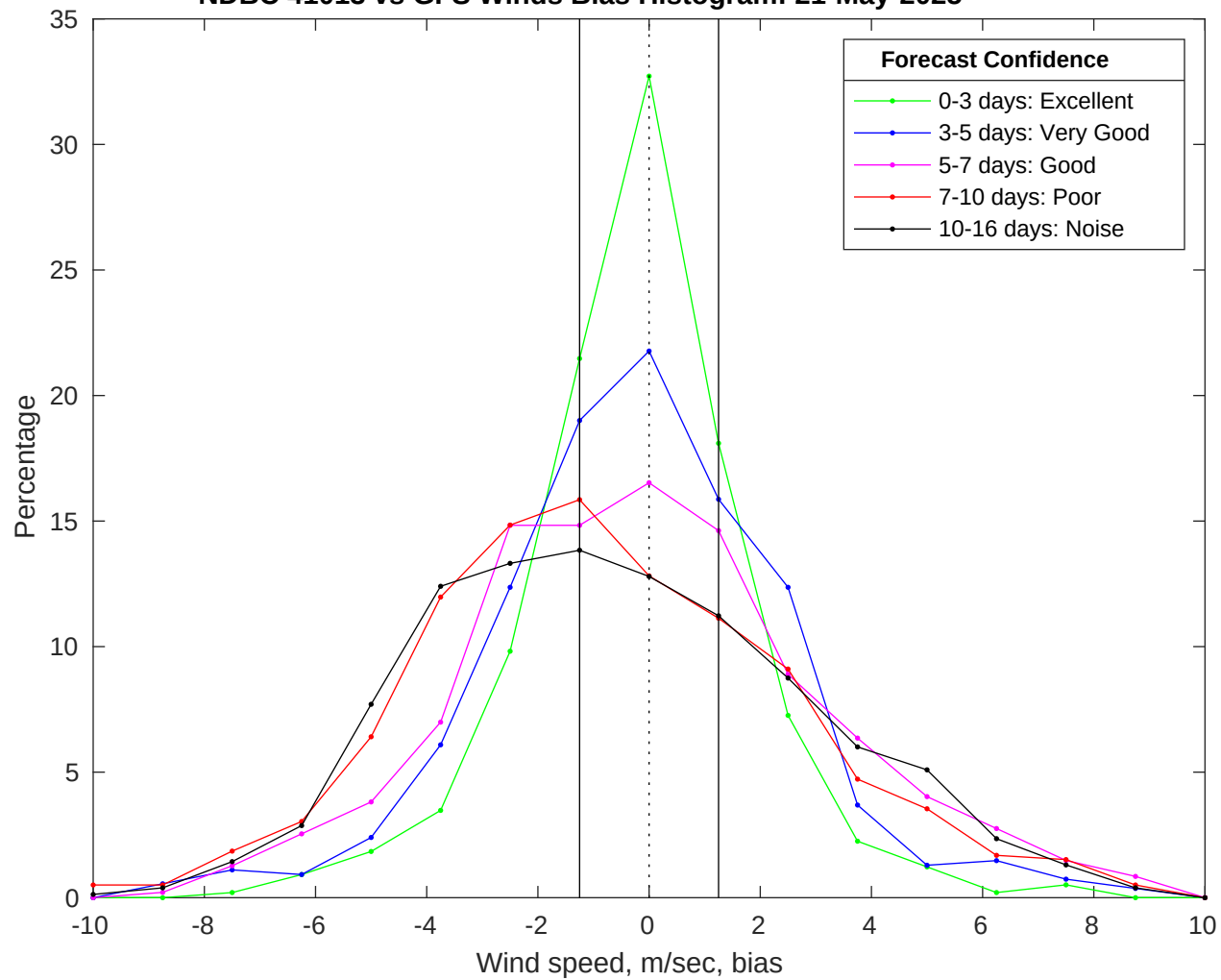
NDBC 41013 vs GFS Winds Bias Histogram: 21-May-2025
