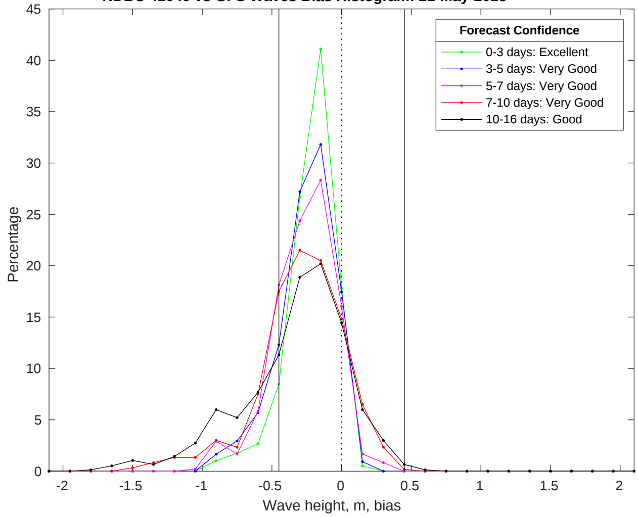
NDBC 41040 vs GFS Waves Bias Histogram: 21-May-2025
