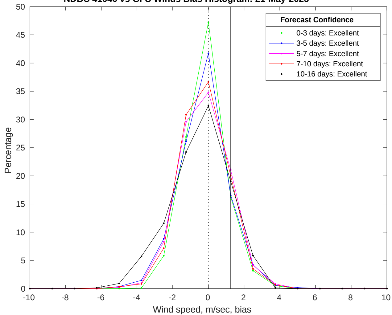
NDBC 41040 vs GFS Winds Bias Histogram: 21-May-2025
