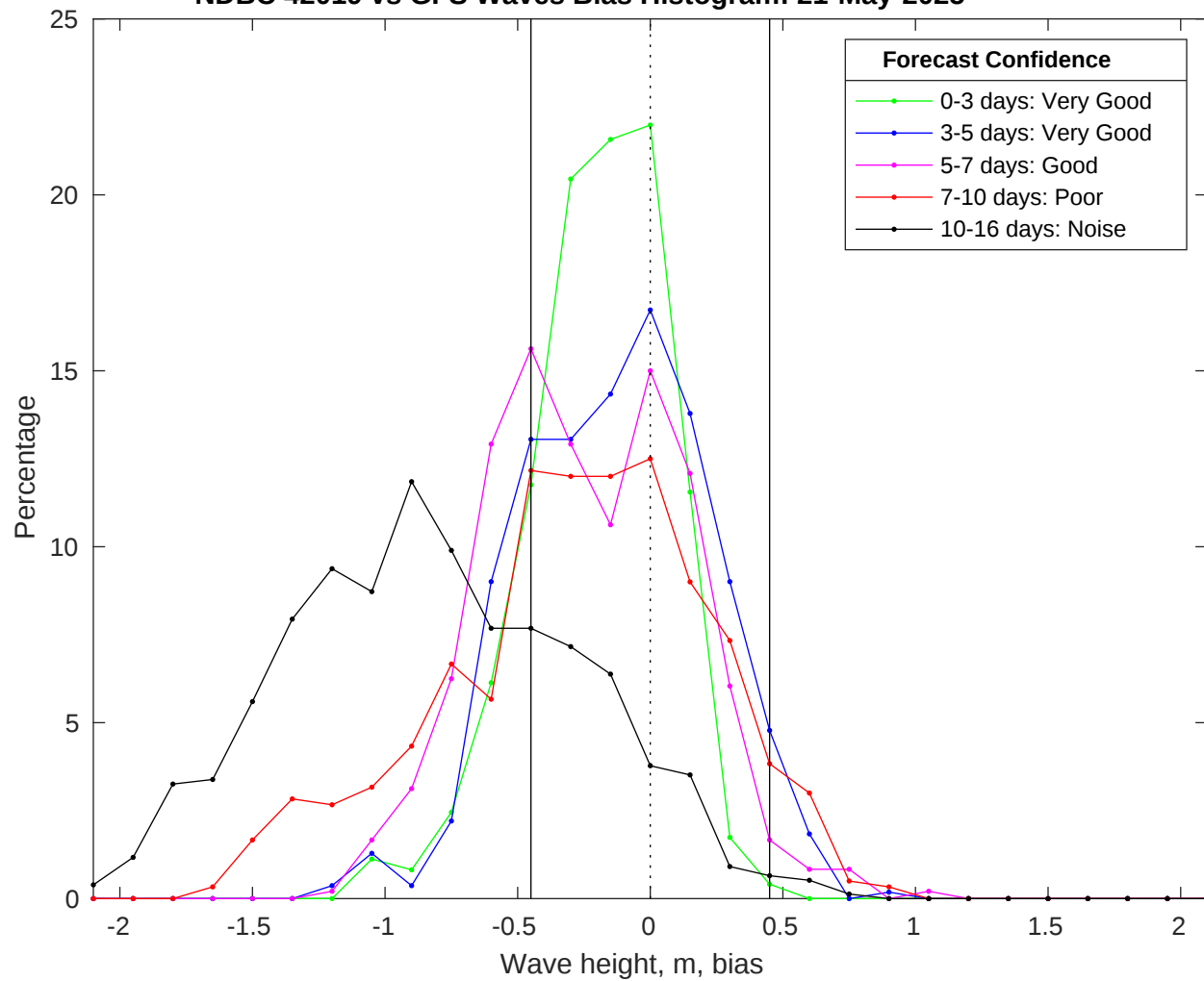
NDBC 42019 vs GFS Waves Bias Histogram: 21-May-2025
