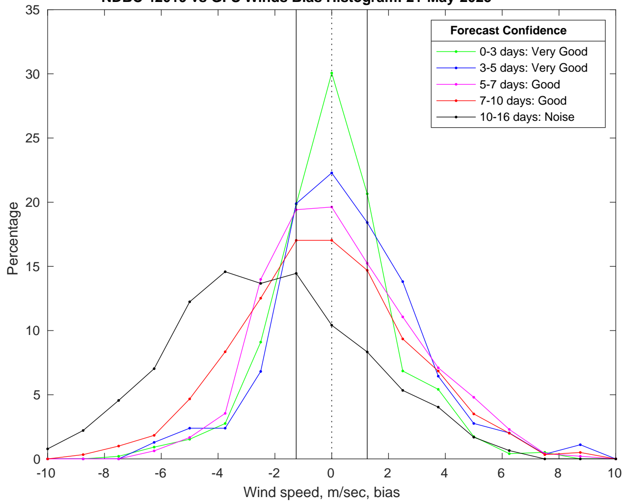
NDBC 42019 vs GFS Winds Bias Histogram: 21-May-2025
