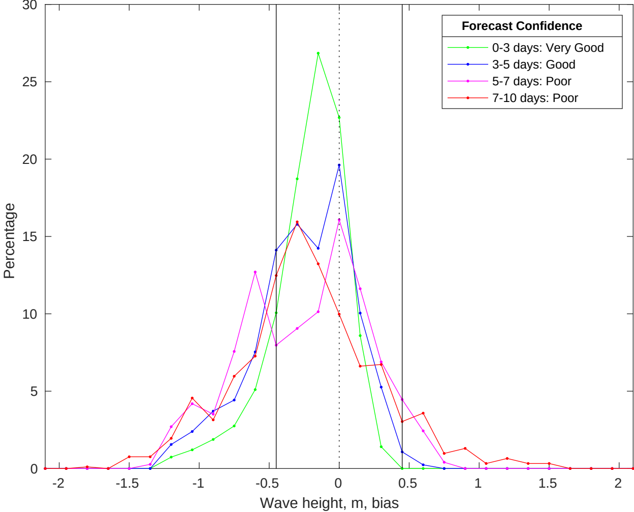
NDBC 42020 vs CMEMS Waves Bias Histogram: 21-May-2025
