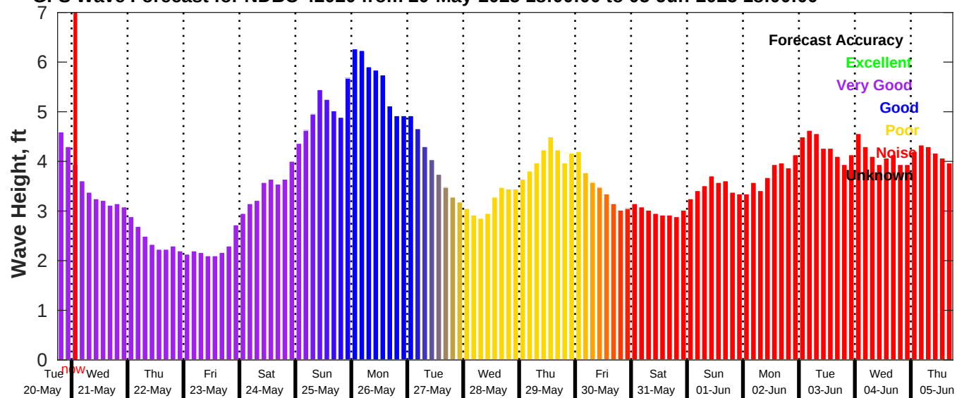
GFS Wave Forecast for NDBC 42020 from 20-May-2025 18:00:00 to 05-Jun-2025 18:00:00
