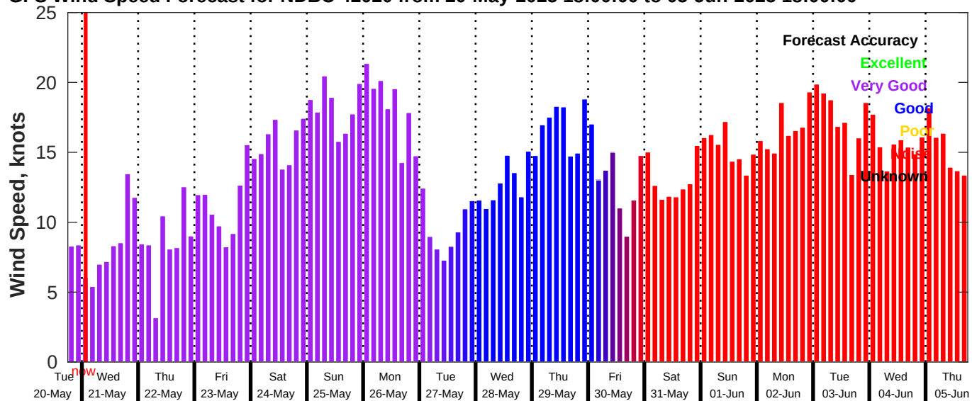
GFS Wind Speed Forecast for NDBC 42020 from 20-May-2025 18:00:00 to 05-Jun-2025 18:00:00
