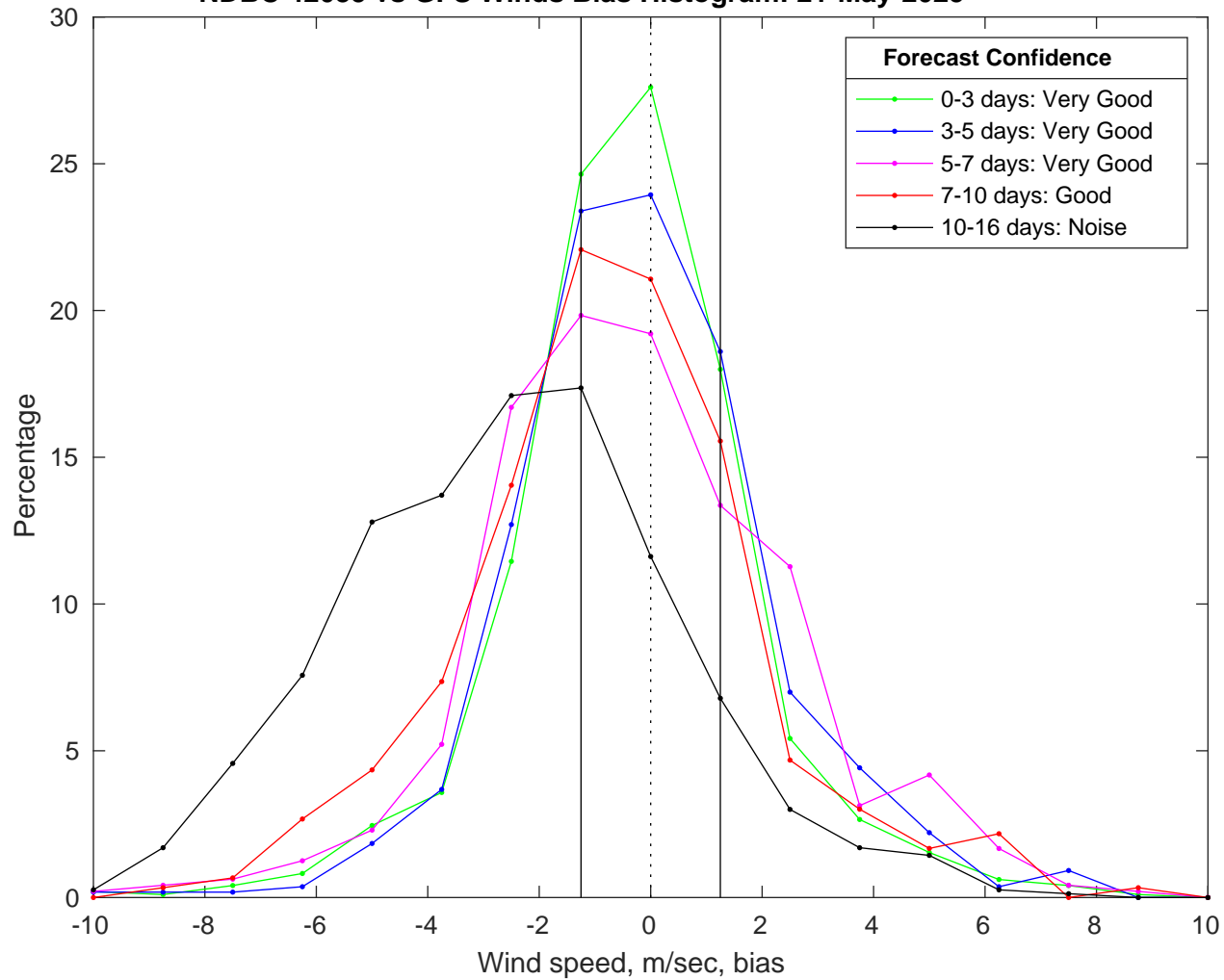
NDBC 42035 vs GFS Winds Bias Histogram: 21-May-2025
