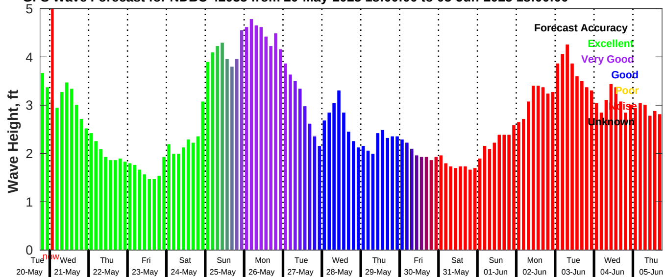
GFS Wave Forecast for NDBC 42035 from 20-May-2025 18:00:00 to 05-Jun-2025 18:00:00
