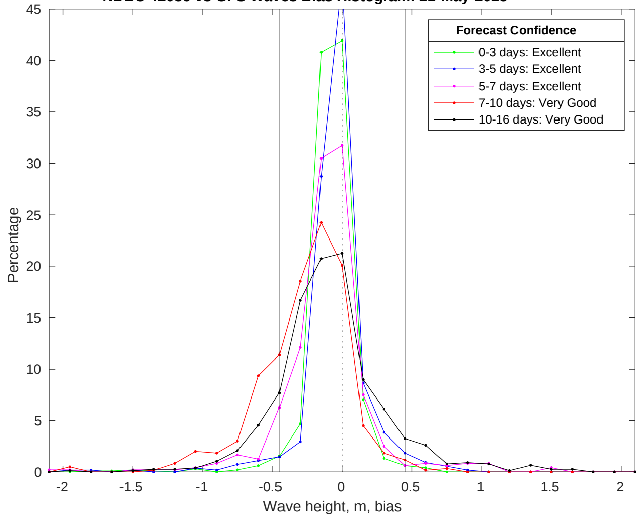
NDBC 42036 vs GFS Waves Bias Histogram: 21-May-2025
