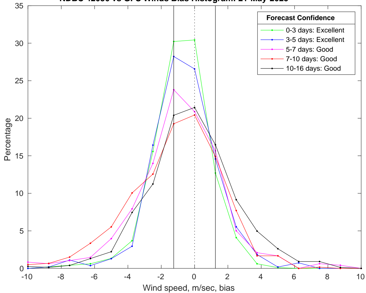
NDBC 42036 vs GFS Winds Bias Histogram: 21-May-2025
